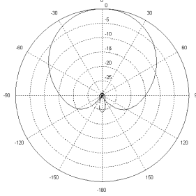
Horizontal Pattern
